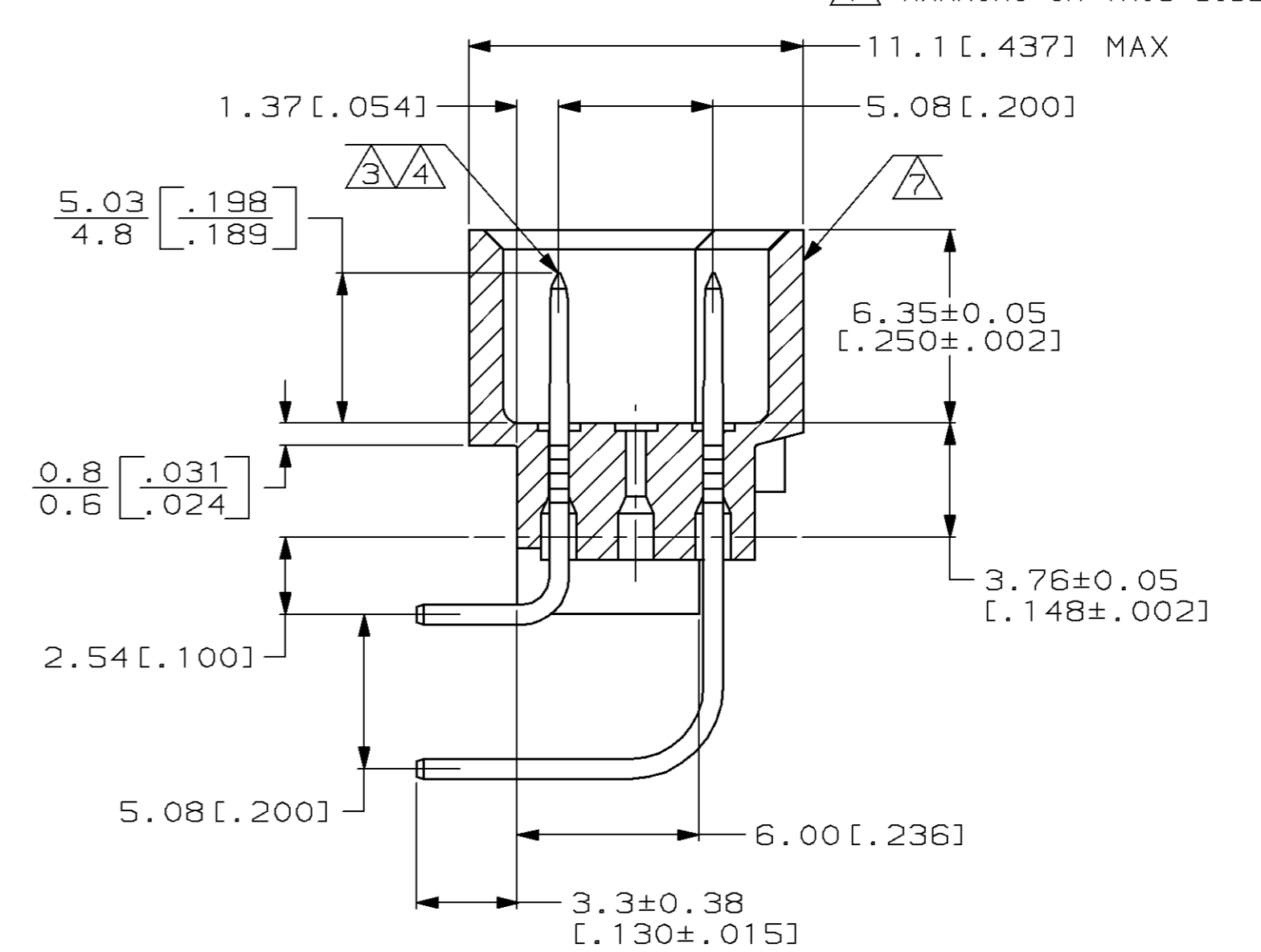
SECTION Z-Z
